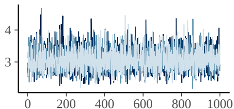
sigma
