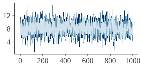
b_Intercept
