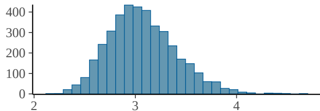
sigma
