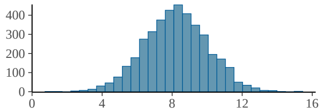
b_Intercept
